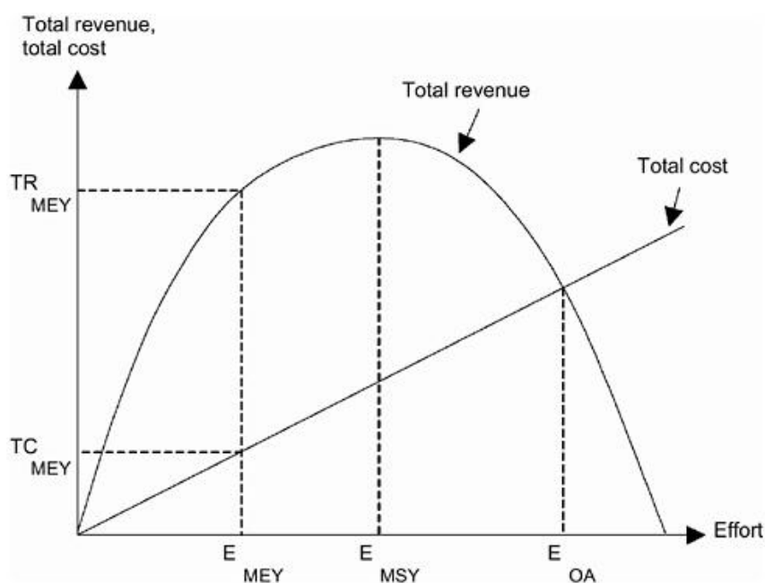
Figure 12. Two-dimensional illustration of a commercial fishery showing MSY, MEY and EY (National Research Council 2002).
